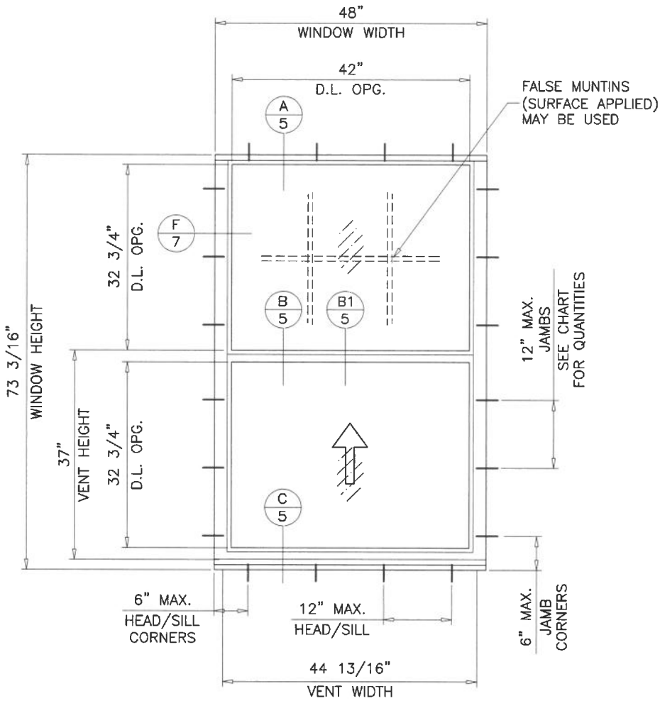
TYPICAL ELEVATION
