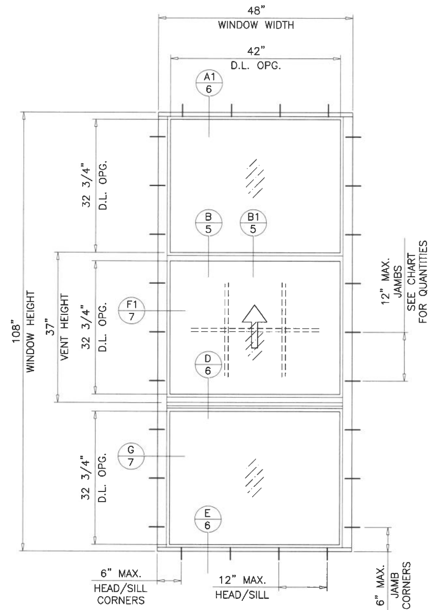
TYPICAL ELEVATION
